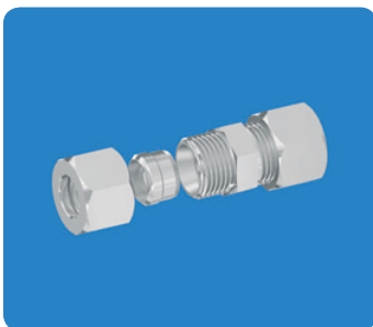
Bite-ring couplings R-1321 PAGE 18
